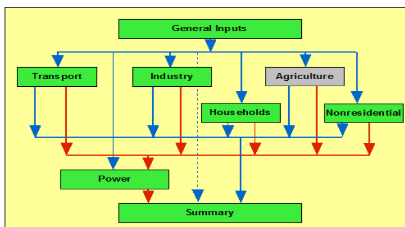
Figure 2: EFFECT Model Structure
