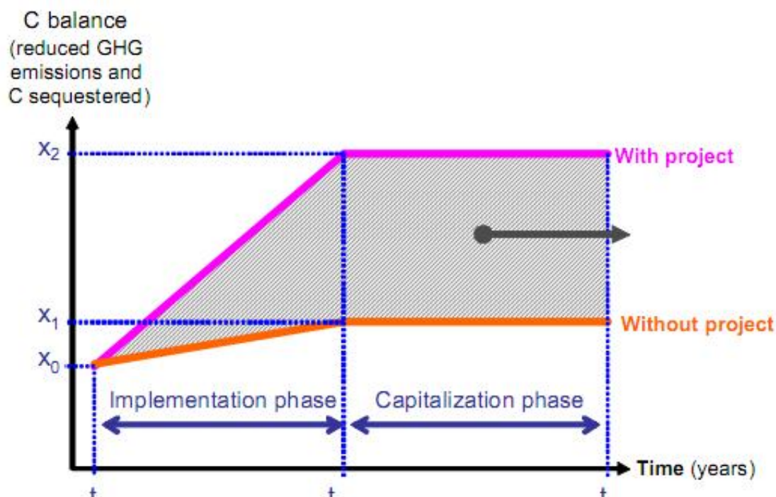
Figure 3: The logic of the Ex-Act tool
