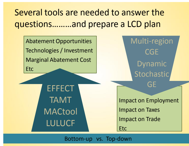
Figure 6: Bottom-up and Top-down Modeling Tools
